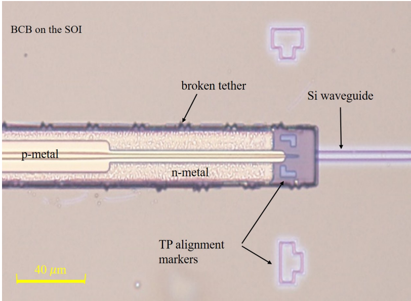
Figure 3.7: Microscope image of a SOA coupon after micro-transfer-printing on SOI.
