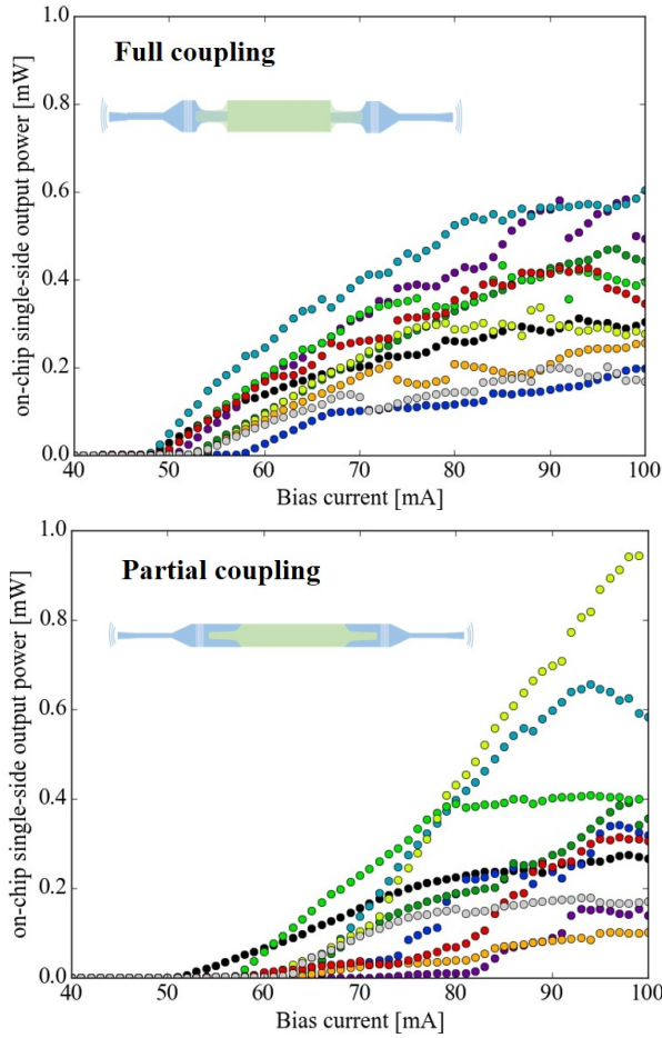
Figure 5.8: Single-sided on-chip output power plotted against bias current for (top) full-coupling and (bottom) partial-coupling design.
