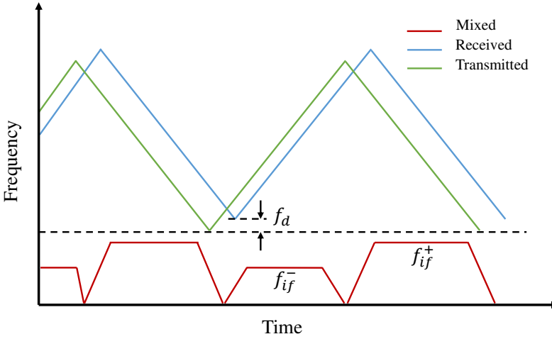
Figure 1.7: An example of received, transmitted and mixed signal in coherent LiDAR system.
