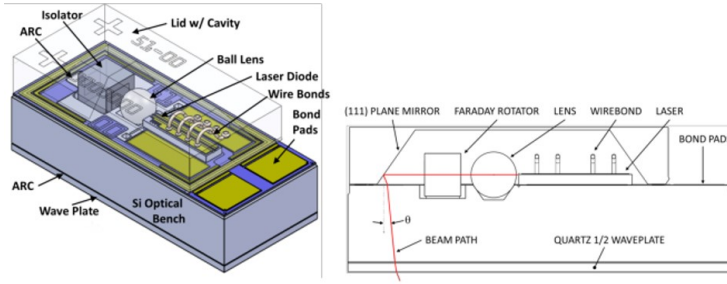
Figure 1.9: Micro-optical bench packaging from Luxtera [29]
