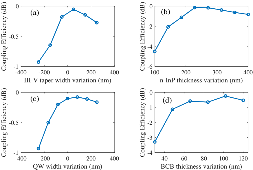
Figure 2.12: (a) Calculated coupling efficiency for variation in (a) adiabatic III-V taper width, (b) n-InP thickness, (c) QW width and (d) BCB thickness.
