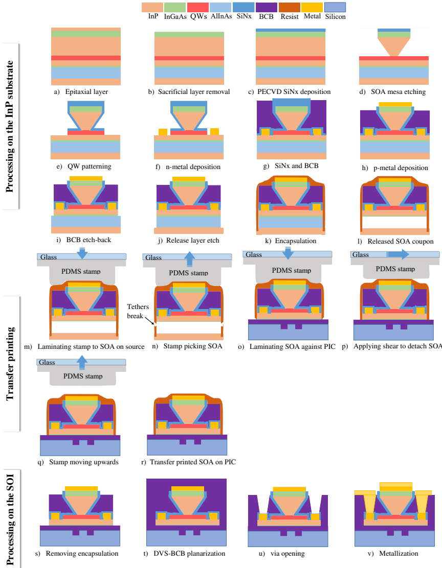
Figure 3.4: The complete process flow of SOA device fabrication which includes patterning on the source InP substrate, micro-transfer-printing, and final processing steps on the SOI target substrate.
