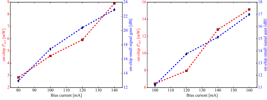
Figure 3.12: The markers represent the fitted values for P_{\text{sat}} and for the small-signal gain G_0 for the full-coupling design (left) and partial-coupling design (right).
