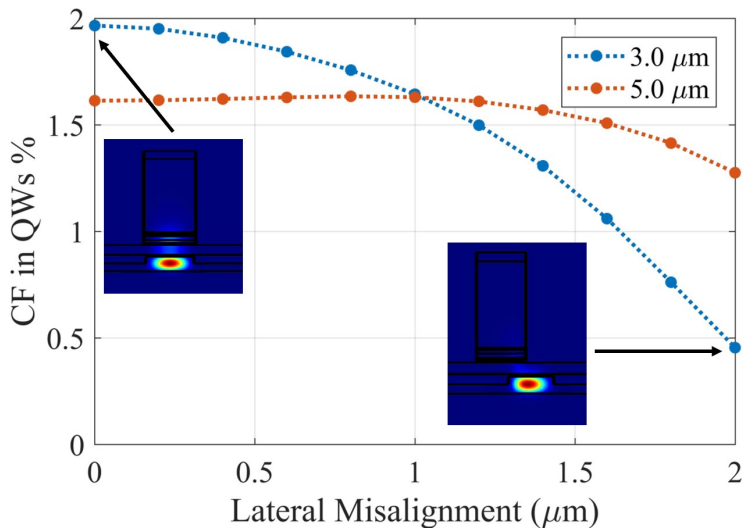
Figure 2.11: The change in confinement factor in QWs with the misalignment variation for 3.0 \mu\text{m} and 5.0 \mu\text{m} Si waveguide width, insets illustrate the mode profile at zero and 2.0 \mu\text{m} misalignment.
