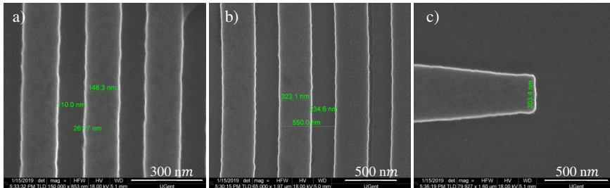
Figure 3.6: a) SEM image of the DBR, b) grating coupler and c) taper tip of the adiabatic taper in Si
