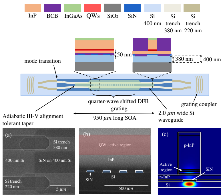
Figure 13: Schematic illustrating the design of the DFB laser with cross-section view of the adiabatic taper and the side view of the DFB grating. SEM images of a) mode transition, b) longitudinal cross-section of the DFB grating and c) the mode profile in the gain section are also shown.
