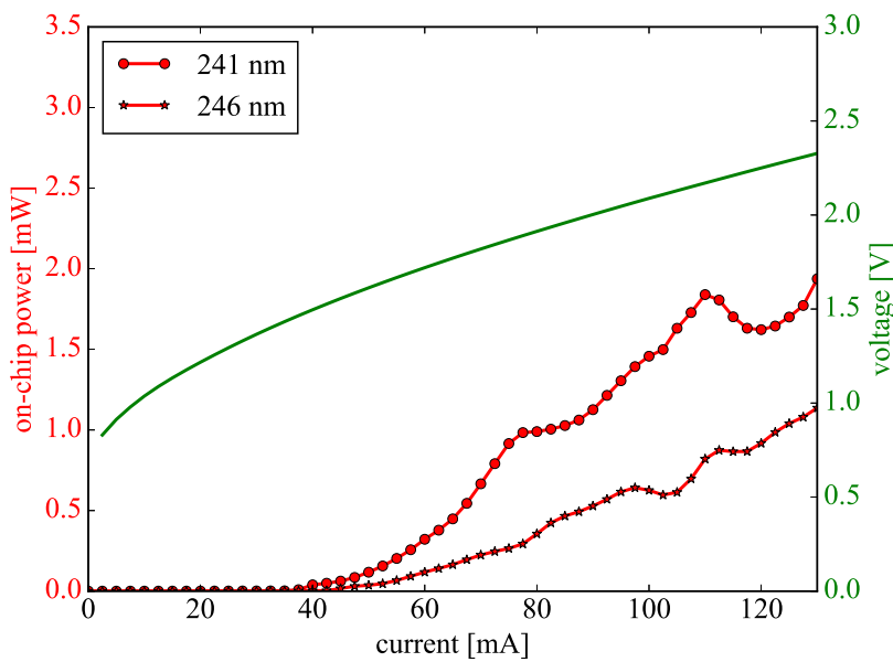
Figure 4.8: Measured on-chip optical power and voltage versus bias current at 20 °C for a grating period of 241 nm and 246 nm.
