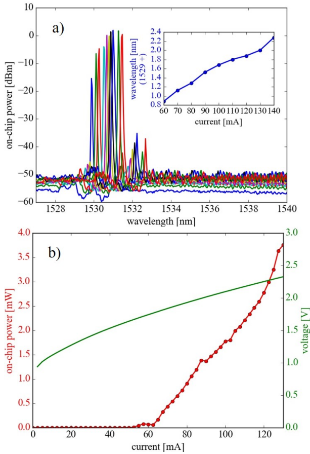
Figure 4.10: (a) Output spectrum at various bias currents, inset illustrates the bias current tuning characteristic of the DFB laser; (b) LI and IV characteristics of the DFB laser.
