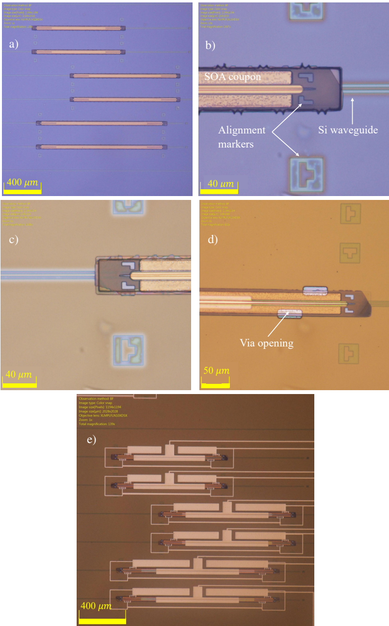
Figure 4.7: (a) Microscope image of SOA coupons micro-transfer printed on SOI, (b) Zoomed-in image (c) after encapsulation removal, (d) after Via opening for n-metal contact and (e) final look after contact metal deposition.
