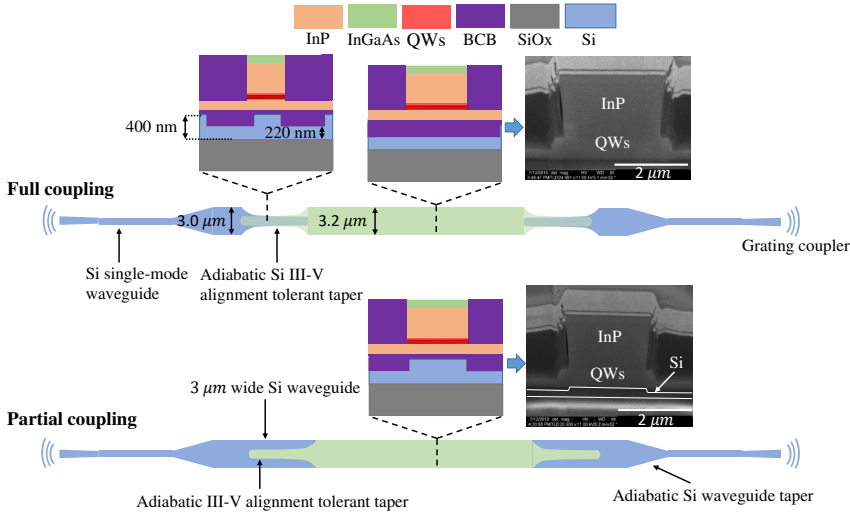
Figure 11: Schematics and FIB cross-sections illustrating the design of the full-coupling and partial-coupling III-V-on-Si SOAs.
