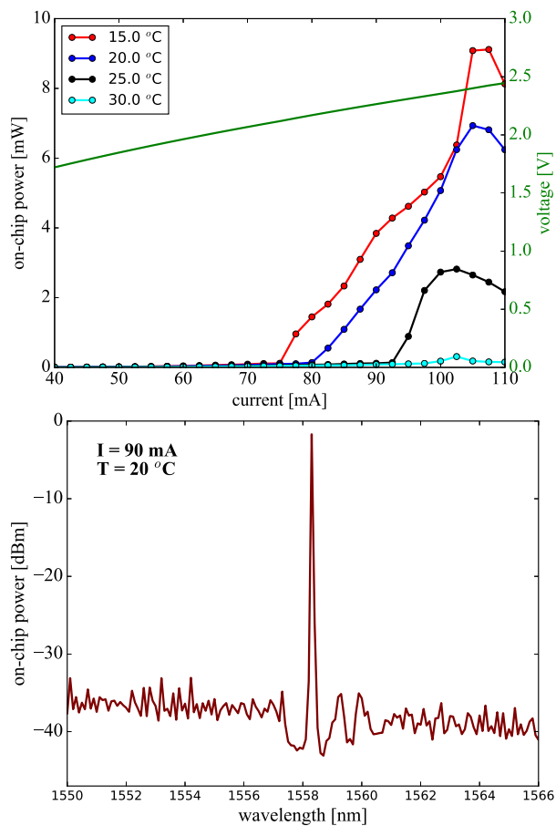
Figure 14: (top) Waveguide-coupled output power (single-sided) as a function of bias current for various operating temperatures and the current-voltage characteristic, (bottom) Measured spectrum at 0.05 nm resolution, at 90 mA and at 20 °C operating temperature.
