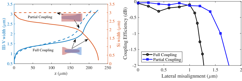
Figure 10: (left) The III-V and Si adiabatic taper width variation along its length. The blue line and the left vertical axis represents the III-V adiabatic taper shape for the partial and full coupling designs. The red line and the right vertical axis represents the Si adiabatic taper shape and Si waveguide width in the case of full coupling and partial coupling, respectively; (right) The simulated coupling efficiency of the adiabatic taper structures for the partial and full-coupling designs versus the lateral misalignment.
