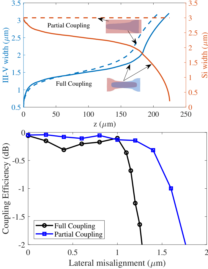
Figure 2.9: (Top) The III-V and Si adiabatic taper width variation along its length. The blue line and the left vertical axis represents the III-V adiabatic taper shape for the partial and full coupling designs. The red line and the right vertical axis represents the Si adiabatic taper shape and Si waveguide width in the case of full coupling and partial coupling, respectively; (Bottom) The simulated coupling efficiency of the adiabatic taper structures for the partial and full-coupling designs versus the lateral misalignment.
