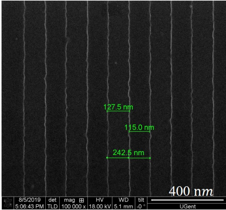
Figure 4.5: SEM image of shallow etched grating
