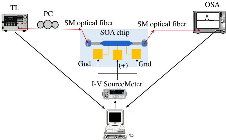
Figure 3.9: The measurement setup used to characterize the SOAs, which includes a tunable laser (TL), polarization controller (PC), optical spectrum analyzer (OSA), and current-voltage source-meter. The computer is used to control the instruments and to process the measured data.
