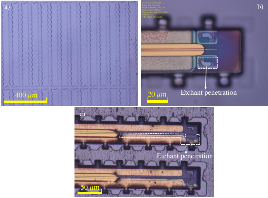
Figure 2.6: (a) Microscope image of a failed release process, the coupons detached from the substrate. b) and c) Microscope image depicting the effects of \text{FeCl}_3 penetration in the SOA coupons.
