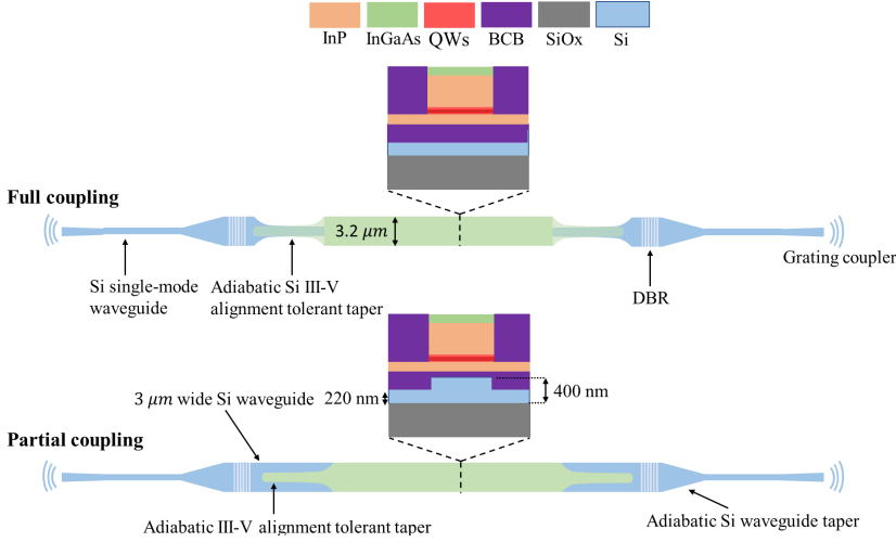
Figure 5.1: a) Design schematic of full-coupling and partial-coupling DBR lasers. The cross-section in the gain section is also illustrated.
