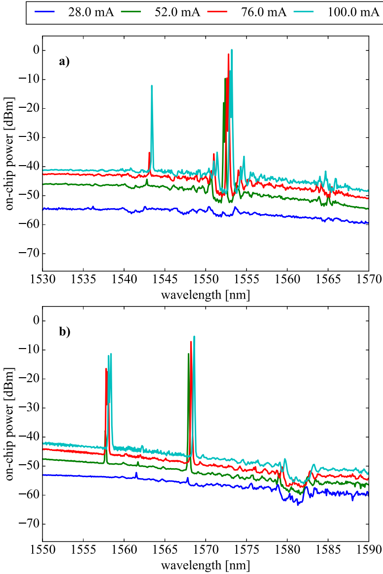
Figure 4.9: Measured spectrum of shallow etch DFB lasers with grating period of (a) 241 nm and (b) 246 nm for various bias currents.
