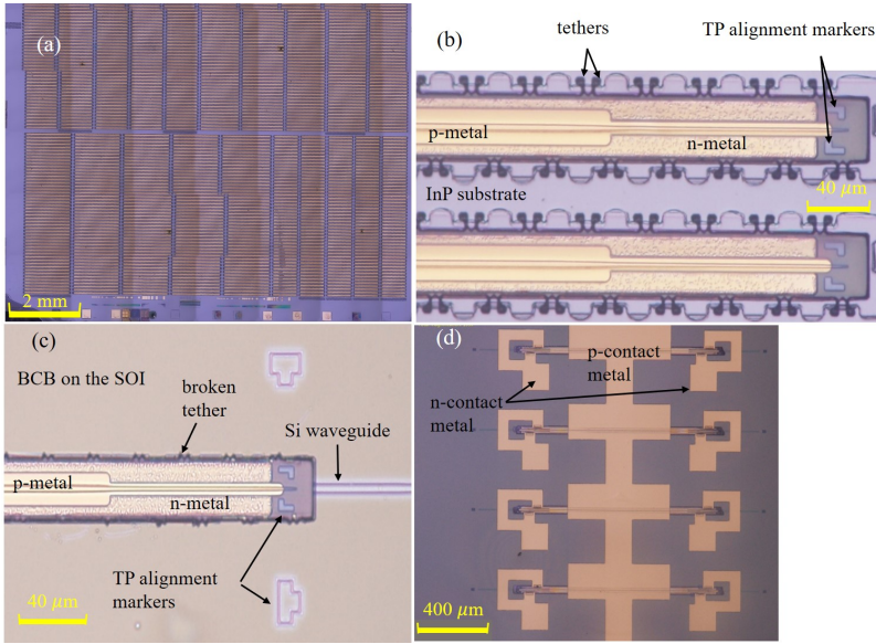
Figure 9: Microscope image of a) processed SOA coupons on the InP substrate, b) two zoomed-in SOA coupons from (a), c) micro-transfer-printed SOA coupon on a Si waveguide, and d) III-V-on-Si SOAs with contact pads.
