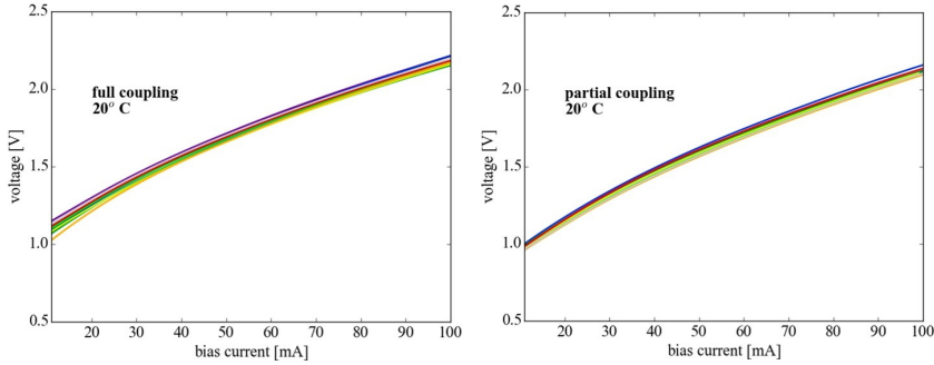
Figure 5.7: Voltage versus bias current for (left) full-coupling design and (right) partial-coupling design.
