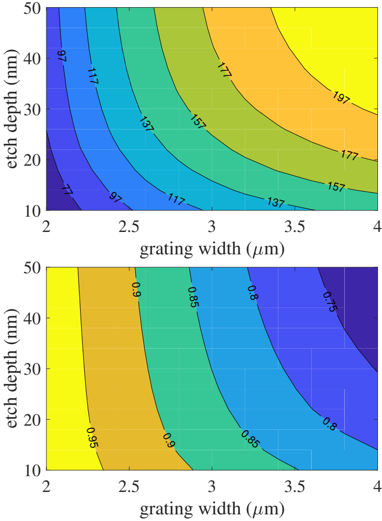
Figure 4.1: (top) Calculated map of \kappa in \text{cm}^{-1} for different widths and etch depths of the grating, (bottom) Calculated map of modal overlap between etched and unetched section of the grating for various grating widths and etch depths.
