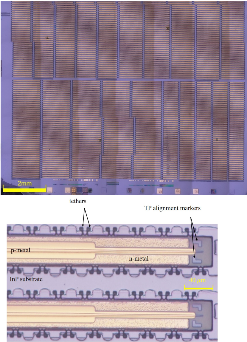
Figure 3.5: (top) Microscope top image of an array of SOA devices patterned and released on the native InP substrate, (bottom) Zoomed-in microscope image of two SOA coupons.
