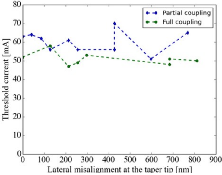
Figure 5.12: DBR lasers threshold current plotted against the lateral misalignment between III-V and Si waveguide.
