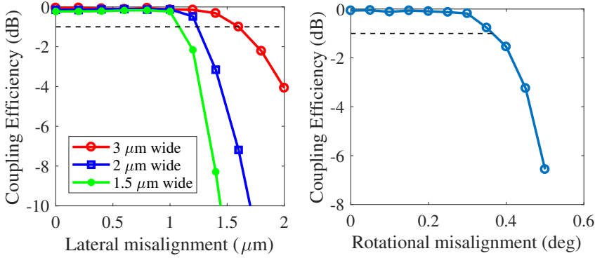
Figure 2.10: (left) Calculated power coupling between full-coupling III-V adiabatic taper design and Si waveguide of width 3.0 \mu\text{m} , 2.0 \mu\text{m} and 1.5 \mu\text{m} , (right) Calculated coupling efficiency against the rotational misalignment between III-V adiabatic taper and Si waveguide.
