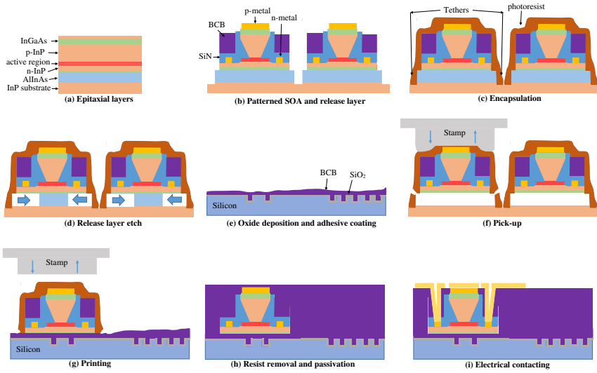
Figure 4.6: Schematic micro-transfer-printing process flow of DFB lasers, (a-d) depicts the processing of SOAs on the InP substrate, (e) illustrates the preparation of the patterned SiPh sample prior to micro-transfer-printing, (f-g) illustrates the picking and printing of the SOAs on the SiPh sample, (h-i) illustrates the post-processing steps on the SiPh sample, which includes passivation and electrical contacting.
