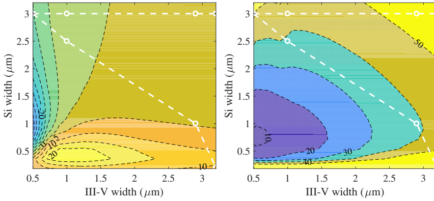
Figure 2.14: Calculated \gamma (left) and \kappa map (right) to design the adiabatic taper for the ISIPP50G platform. The white dashed lines represent the selected III-V and Si width combinations for the full-coupling and partial-coupling designs.
