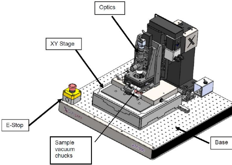
Figure 2.7: Schematic of the \mu TP-100 lab scale printer.
