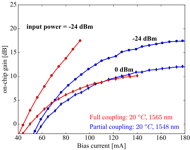
Figure 3.10: The variation of on-chip gain with the bias current at lower on-chip input power of -24 dBm and higher on-chip input power of 0 dBm for both the full-coupling (in red) and partial-coupling (in blue) SOA design.
