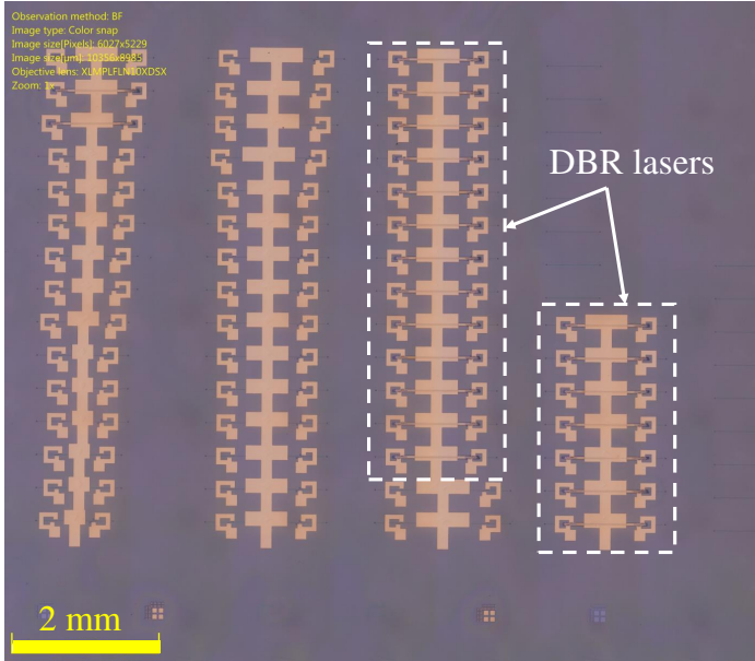
Figure 5.6: Array of DBR lasers on the III-V-on-silicon die.
