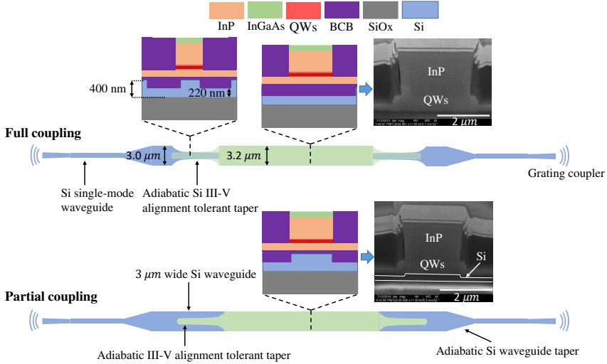
Figure 3.1: Schematics and FIB cross-sections illustrating the design of the full-coupling and partial-coupling III-V-on-Si SOAs.
