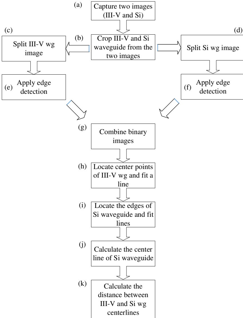
Figure 5.13: Process flow chart of misalignment measurement from the microscope images of micro-transfer printed SOAs.
