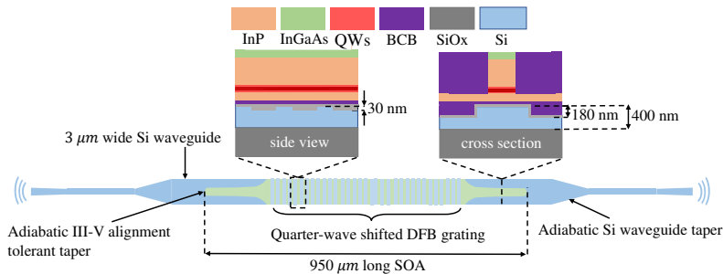
Figure 4.2: Schematic illustrating the design of the DFB laser, the cross-section view of the adiabatic taper and the side view of the DFB grating.
