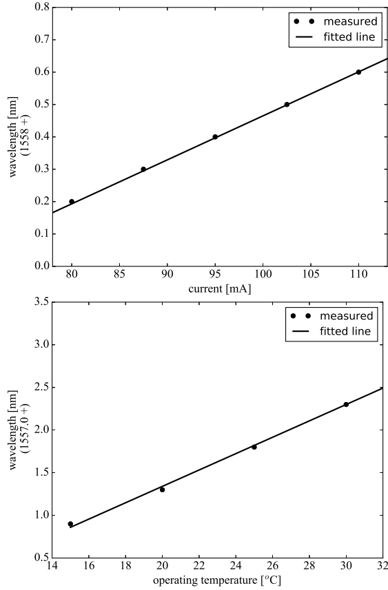
Figure 4.15: DFB output-wavelength-tuning characteristics (top) with changing bias current at 20 °C and (bottom) with changing operating temperature at 90 mA.
