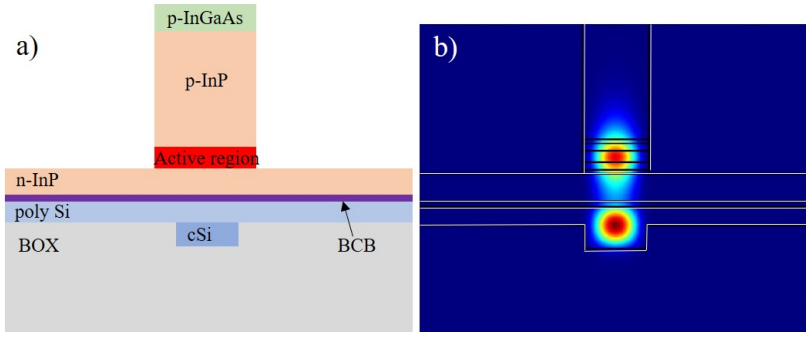
Figure 2.13: Schematic illustration and simulated mode profile of the ISIPP50G waveguide cross-section with integrated SOA.
