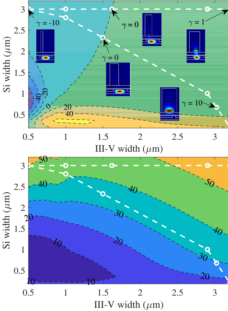
Figure 2.8: (Top) Calculated map of \gamma for several width combinations of the III-V and Si waveguide. The white dashed lines represent the trajectory of the points chosen to design the adiabatic tapers. The insets are the optical modal profiles found using simulations at \gamma = -10 (the optical mode is mostly confined in the Si waveguide), \gamma = 0 (this is the phase matching point at which the coupling takes place), \gamma = 1 (the optical mode is distributed unevenly in both Si and III-V waveguide), and \gamma = 10 (the optical mode is confined in the III-V waveguide), (Bottom) Calculated map of \kappa in \text{mm}^{-1} for several width combinations of the III-V and Si waveguide.
