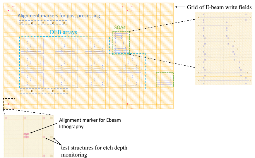
Figure 4.3: Schematic illustrating the DFB SOI layout designed for processing with e-beam.
