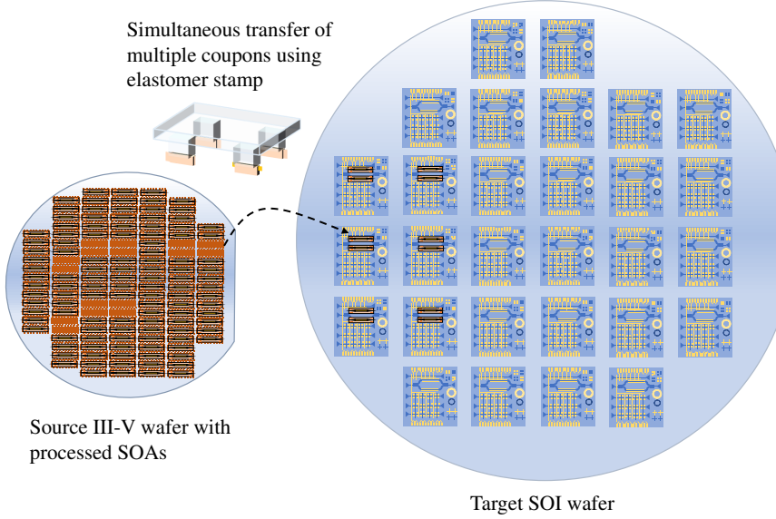
Figure 2.1: Schematic illustrating the micro-transfer printing of four SOA coupons to a SOI wafer using a PDMS stamp.
