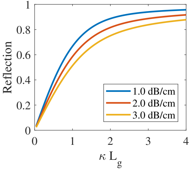
Figure 5.3: Fraction of power reflected is plotted against the grating strength for several values of waveguide loss.
