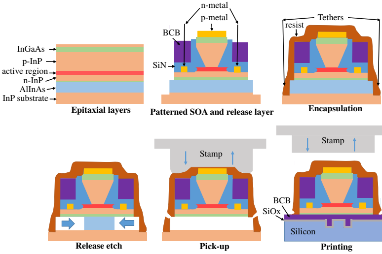
Figure 8: Schematic illustrating the micro-transfer printing process of pre-processed SOA coupons.
