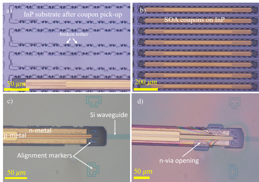
Figure 5.5: a) Image of the InP die after coupons have been picked for micro-transfer printing, b) array of SOA coupons fabricated on the InP die, c) Micro-transfer printed SOA coupon on a Si waveguide and d) opening of n-vias for n-metal deposition.
