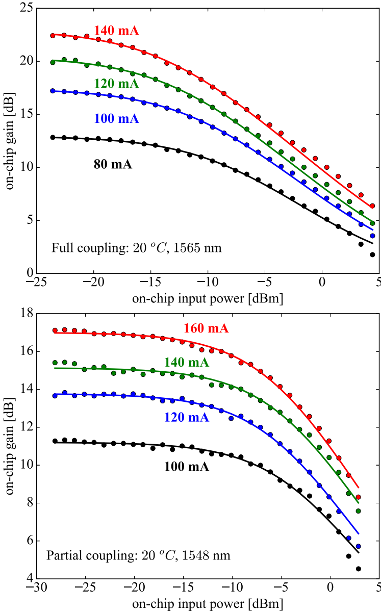
Figure 3.11: Variation of the on-chip gain with the on-chip input power for various bias currents, (top) for the full-coupling design at 1565 nm, (bottom) for the partial-coupling design at 1548 nm. Data points represent the measured values and the solid lines are a fitting with Eq. (3.1).
