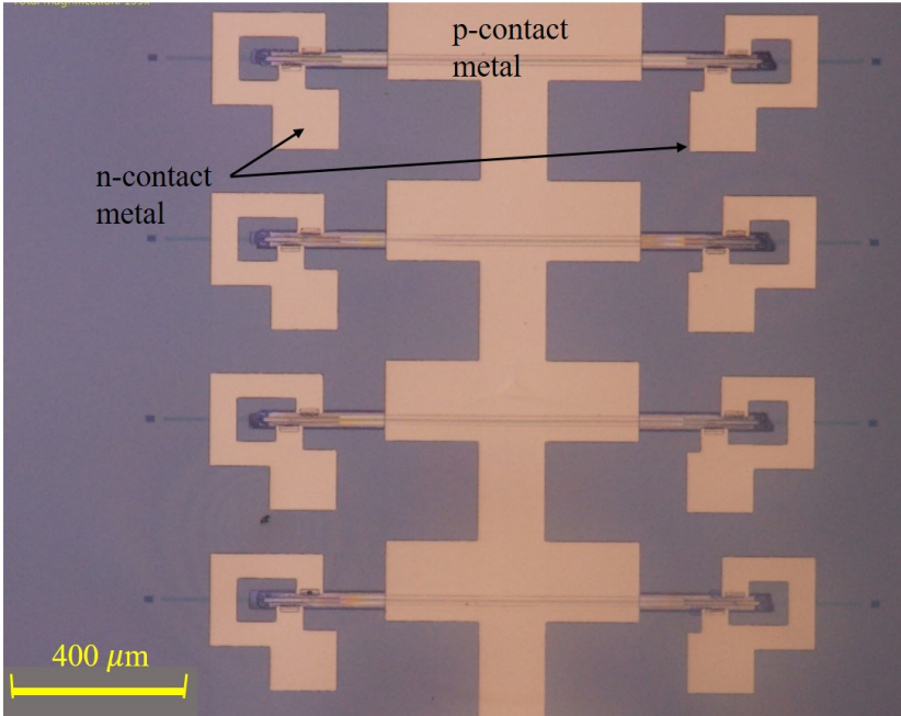
Figure 3.8: Microscope image after contact metal deposition on the SOI.
