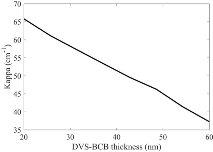
Figure 4.12: DVS-BCB variation with respect to change in \kappa
