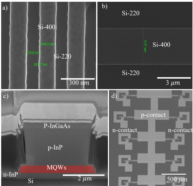
Figure 5.4: SEM images of the fabricated lasers: (a) Zoomed-in images of the DBR, (b) Si waveguide in the gain section for the partial coupling design, (c) Cross-section of the laser in the gain section for the full-coupling design and (d) Final look after contact metal deposition.
