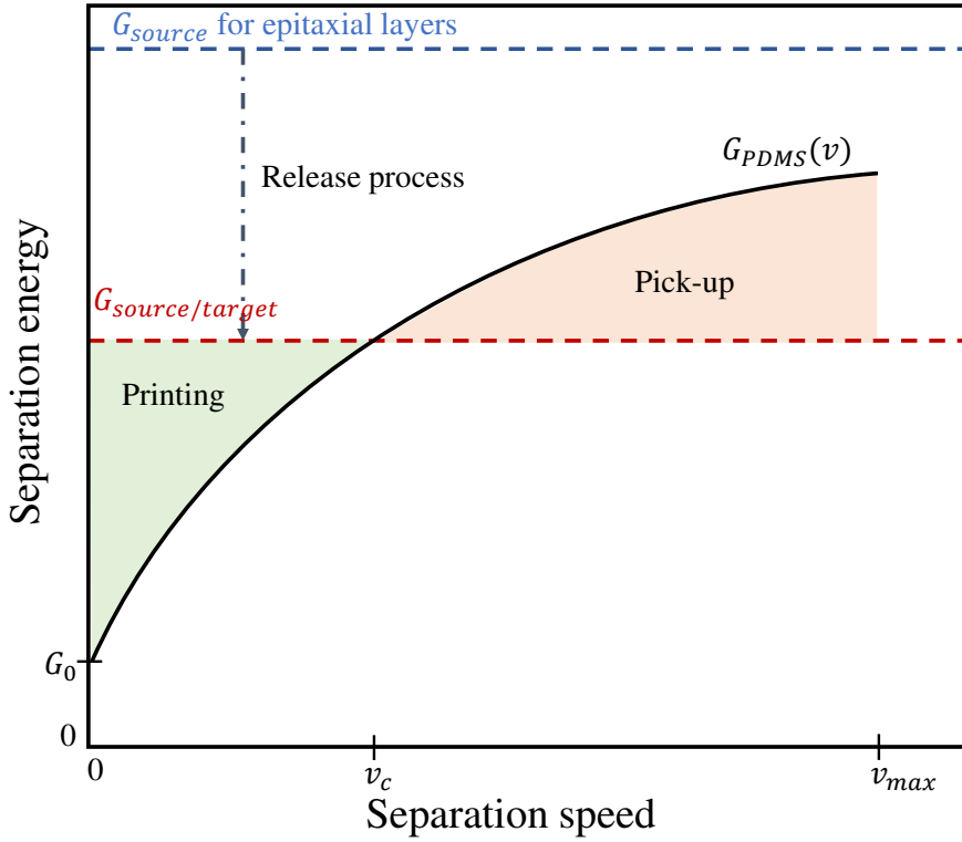
Figure 2.2: Schematic illustrating the dependence of separation energy on the separation velocity of the PDMS stamp. The blue dotted line shows the high separation energy of semiconductor epitaxial layers. For simplicity we assume that G_{source} = G_{target} in this graph.
