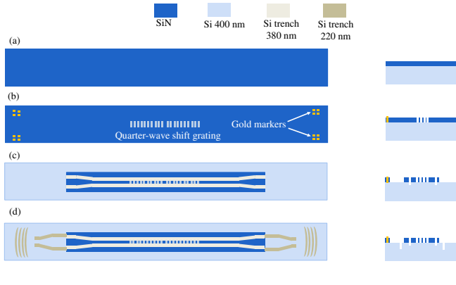
Figure 4.13: DFB with SiN grating process flow: a) SiN deposition, b) patterning of DFB grating and gold marker deposition, c) patterning of 380 nm thick Si trench, d) patterning of 220 nm thick Si trench and grating couplers.
