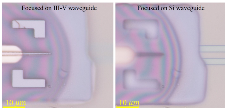
Figure 5.9: 10x magnification microscope images of III-V and Si waveguide.
