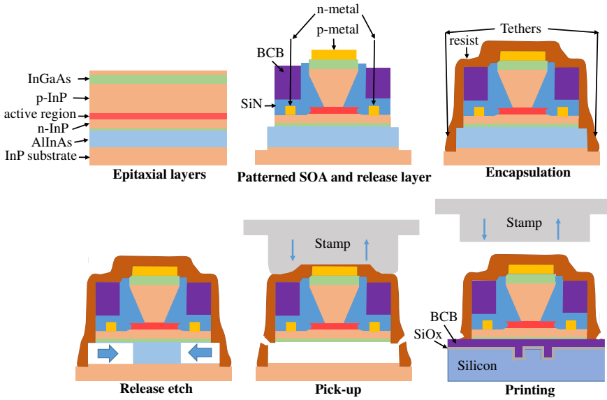
Figure 2.3: Schematic illustrating the micro-transfer printing process of processed SOA coupons.
