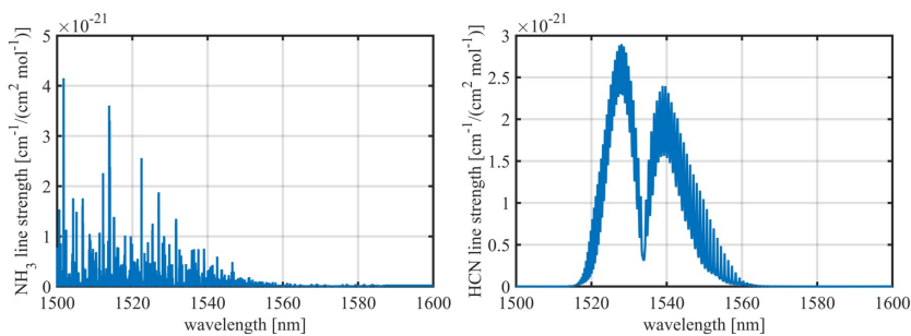
Figure 1.4: Absorption spectra of pure NH 3 and HCN (100 % by volume) in the NIR spectral region at 273 K and 1 atm pressure.
