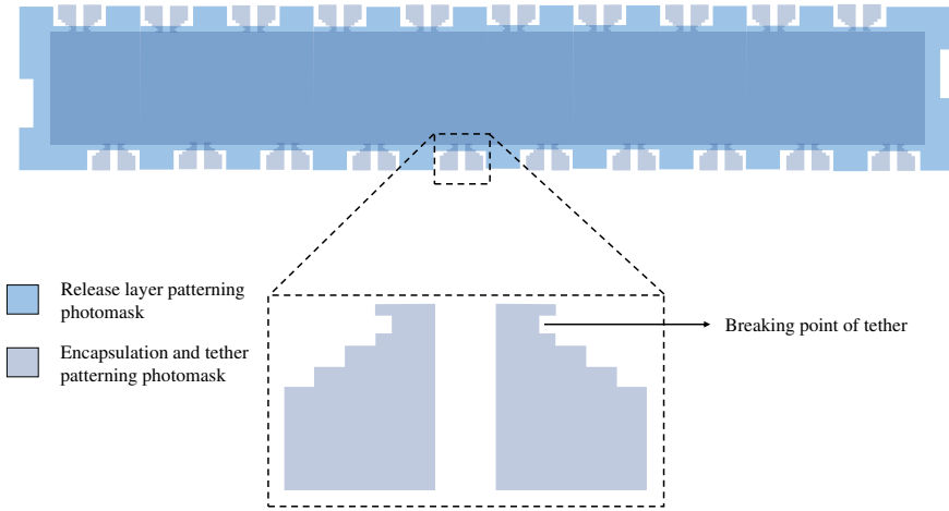
Figure 2.4: Schematic illustrating the photomask used to pattern the release layer and to encapsulate the device. The zoom-in schematic of the tether design is also depicted.
