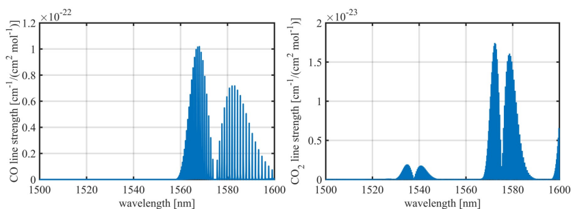
Figure 1.3: Absorption spectra of pure CO and CO 2 (100 % by volume) in the NIR spectral region at 273 K and 1 atm pressure.
