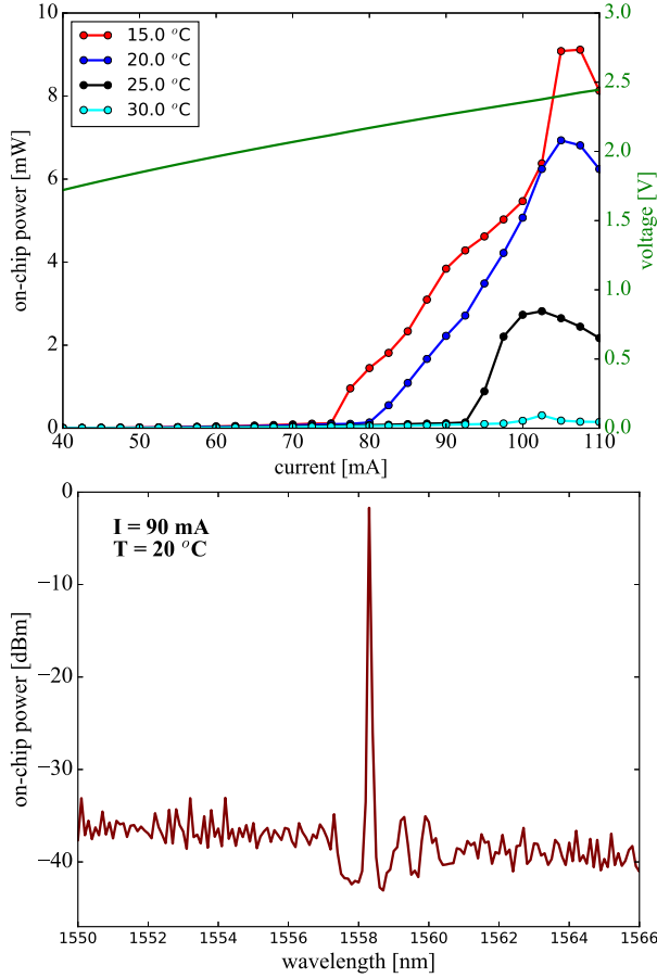
Figure 4.14: (top) Waveguide-coupled output power (single-sided) as a function of bias current for various operating temperatures and the current-voltage characteristic, (bottom) Measured spectrum at 0.05 nm resolution, at 90 mA and at 20 °C operating temperature.
