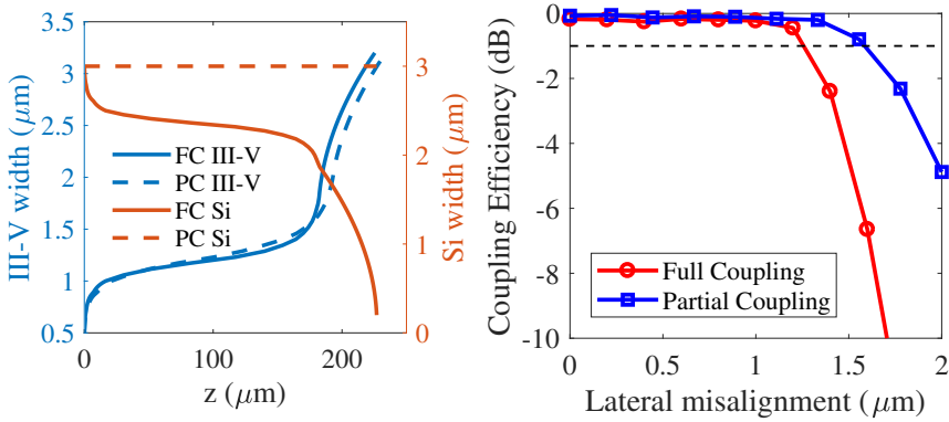
Figure 2.15: (left) Designed shape of the adiabatic alignment tolerant tapers. The full-coupling design and partial-coupling design is represented by the solid curves and the dashed curves, respectively.
