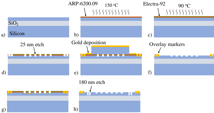
Figure 4.4: a) 400 nm SOI wafer, b) Spin coating of ARP-6200.09 e-beam resist and baking at 150 °C, c) Spin coating of charge reduction layer Electra-92 at 90 °C, d) Development of the e-beam resist and etching in RIE, e) Ti/Au deposition after covering the chip with a Si piece, f) Lift-off and resist removal, g) Repeat step (a-d), h) Final look at the SOI sample with two etching steps.
