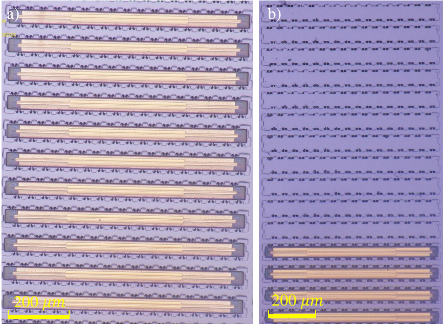
Figure 2.5: a) Microscope image of the released SOA coupons, b) Microscope image of the sample after coupons have been picked-up.
