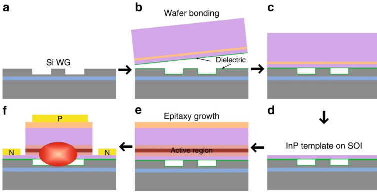
Figure 1.8: Process flow schematic of regrowth on a bonding template III-V-on-Si integration [24]
