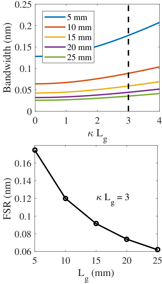
Figure 5.2: (top) Null bandwidth of the DBR is plotted against \kappa L_g for different grating lengths, (bottom) The FSR of the FP cavity (assuming a 1mm long SOA) for different lengths of the highly reflective grating.
