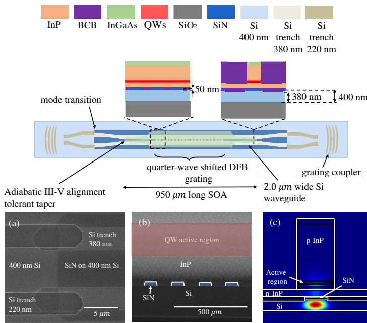
Figure 4.11: Schematic illustrating the design of the DFB laser with cross-section view of the adiabatic taper and the side view of the DFB grating. SEM images of a) mode transition, b) longitudinal cross-section of the DFB grating and c) the mode profile in the gain section are also shown.
