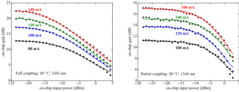
Figure 12: Variation of the on-chip gain with the on-chip input power for various bias currents, (left) for the full-coupling design at 1565 nm, (right) for the partial-coupling design at 1548 nm.
